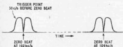
Fig. 2. Output amplitude/time characteristic of amplifier (9) during operation.
